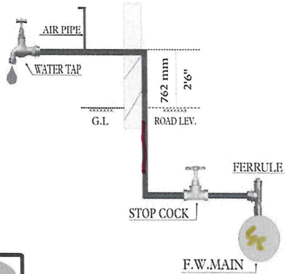
DETAILS OF FEEDING POINT
